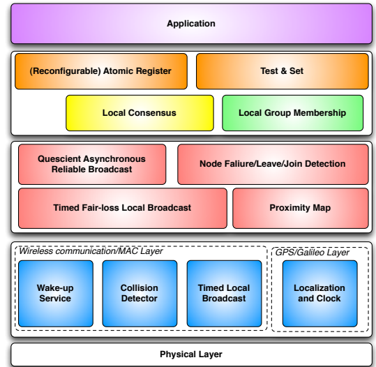
Figure 1: FADA architectural description
